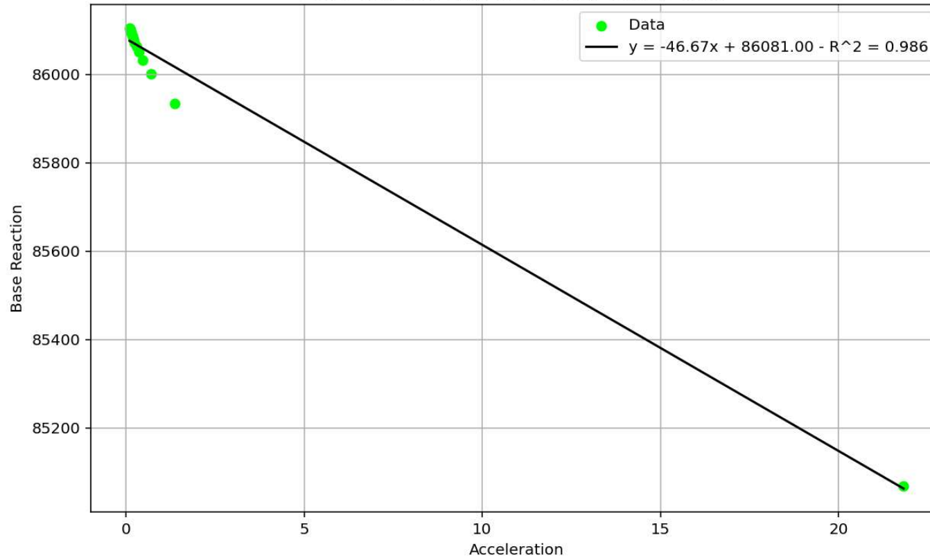
Base Reaction and Acceleration scatter chart
