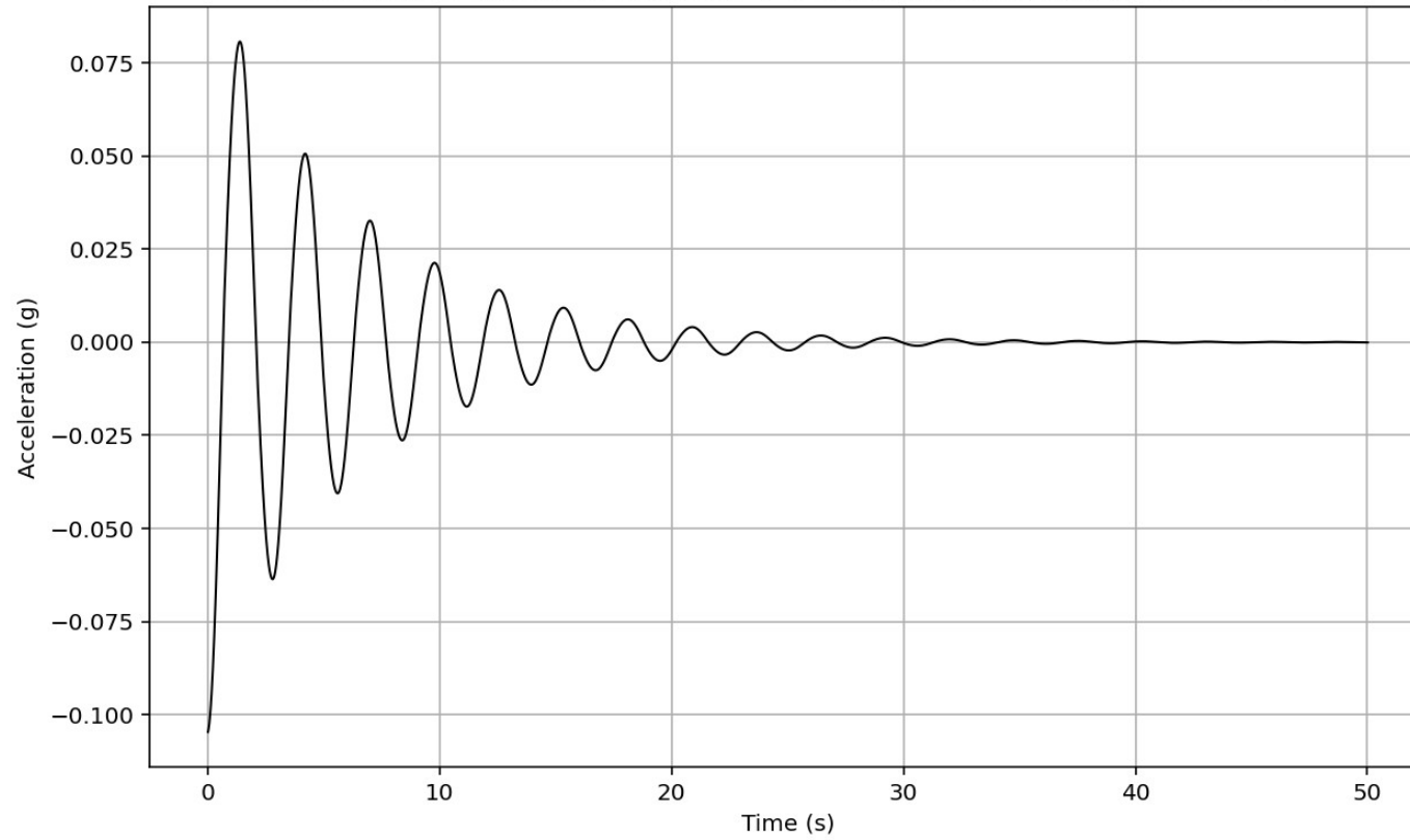
Last Analysis Structural Response + Ground Motion ::: MAX. ABS. : 0.1047
