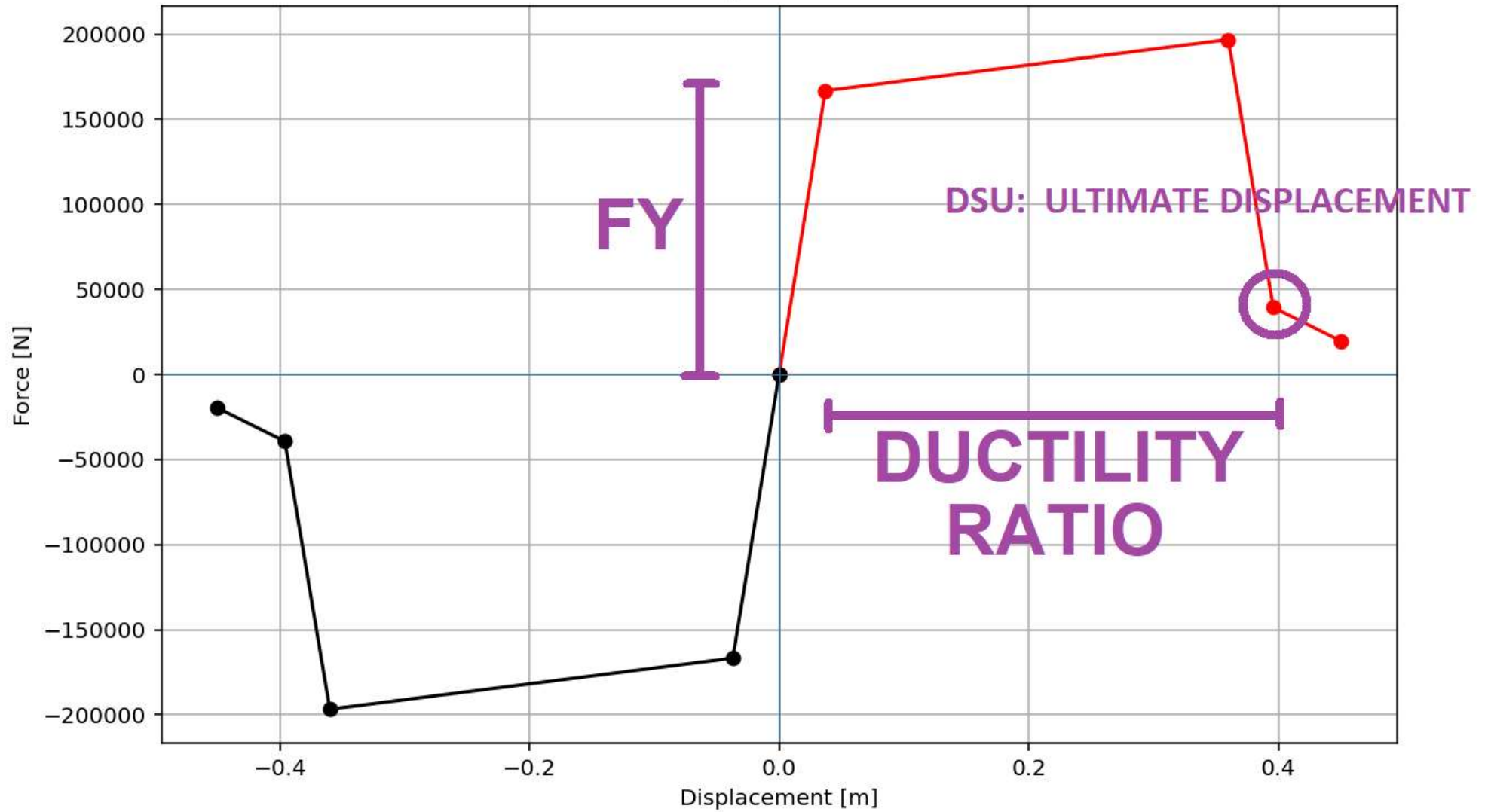
Force-Displacement Curve
