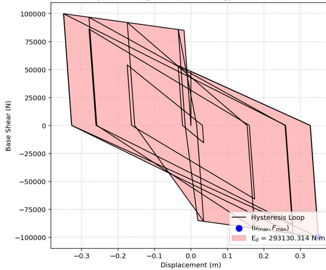
Cyclic Loading - Dissipated Energy (Convex Hull)
