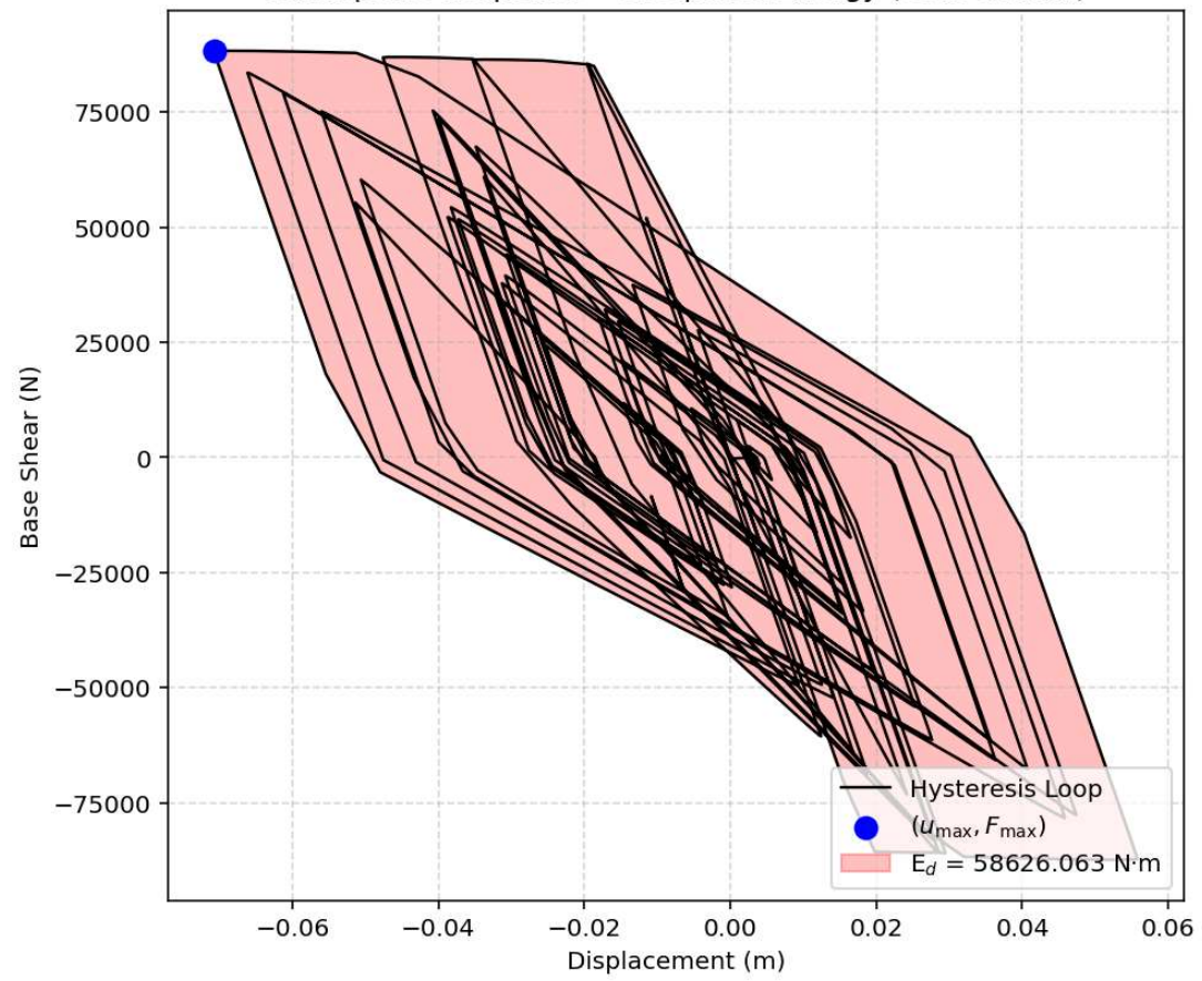
Earthquake Response - Dissipated Energy (Convex Hull)
