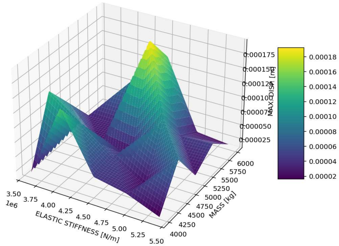
3D CONTOUR: ELASTIC STIFFNESS [N/m] - MASS [kg] - MAX. DISP. [m]
