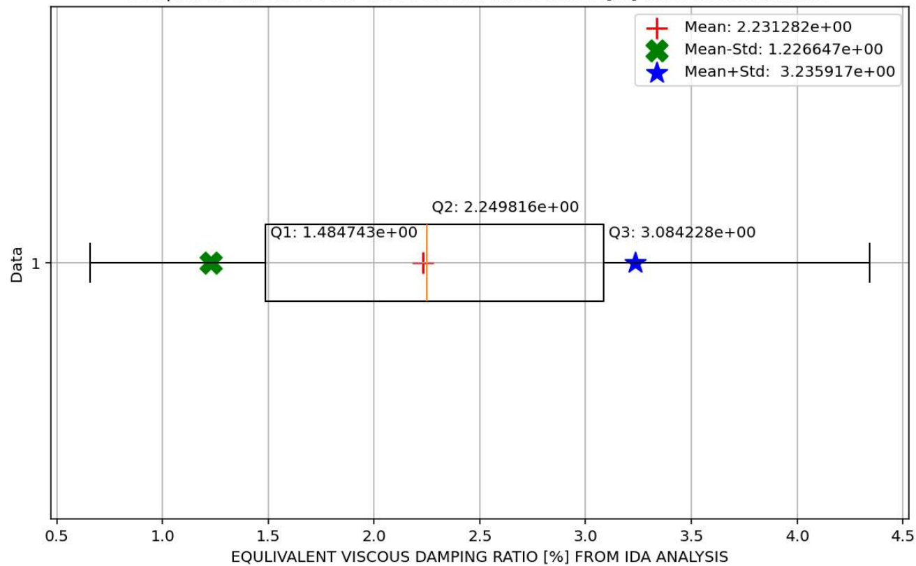
Boxplot of EQUIVALENT VISCOUS DAMPING RATIO [%] FROM IDA ANALYSIS
