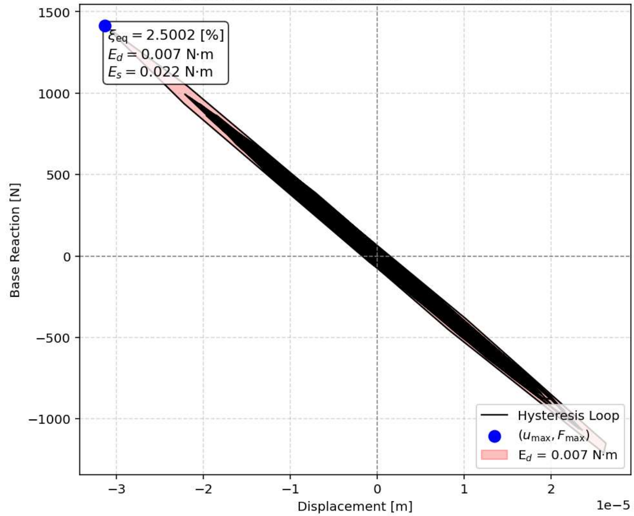
Equivalent viscous damping ratio - Seismic Hysteresis
