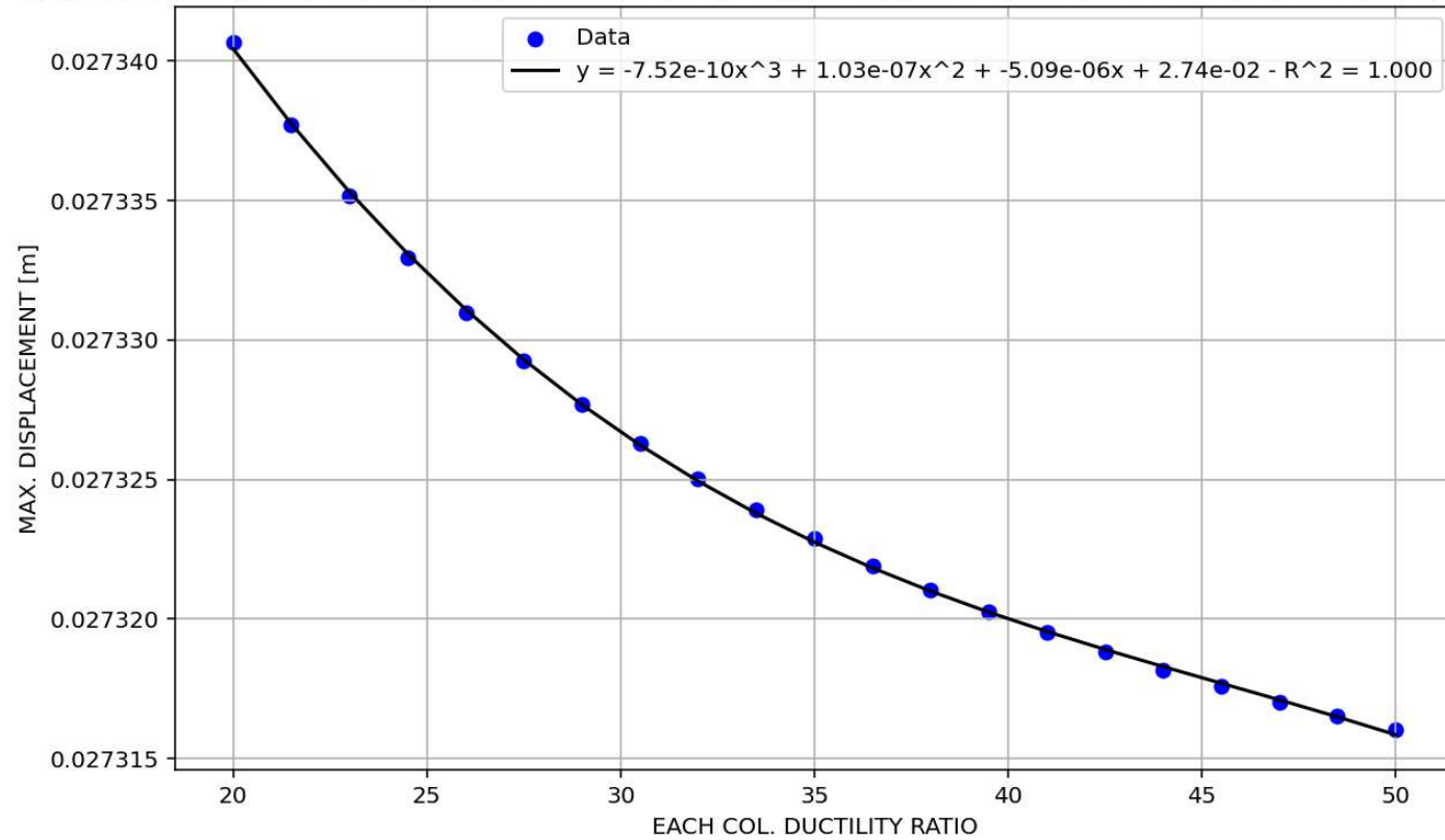
MAX. DISPLACEMENT [m] and EACH COL. DUCTILITY RATIO DURING PERIOD ANALYSIS WITH 20 GROUND MOTIONS
