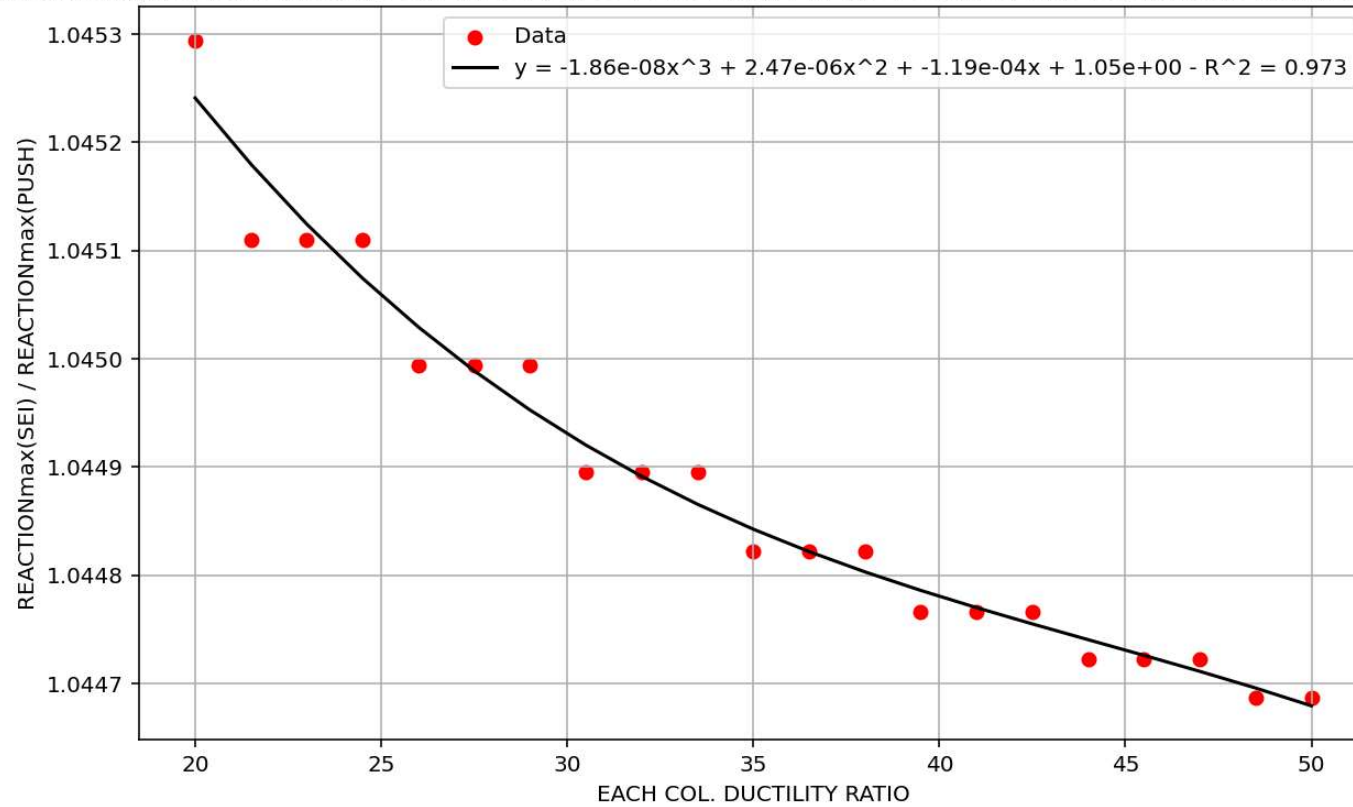
REACTIONmax(SEI) / REACTIONmax(PUSH) and EACH COL. DUCTILITY RATIO DURING PERIOD ANALYSIS WITH 20 GROUND MOTIONS
