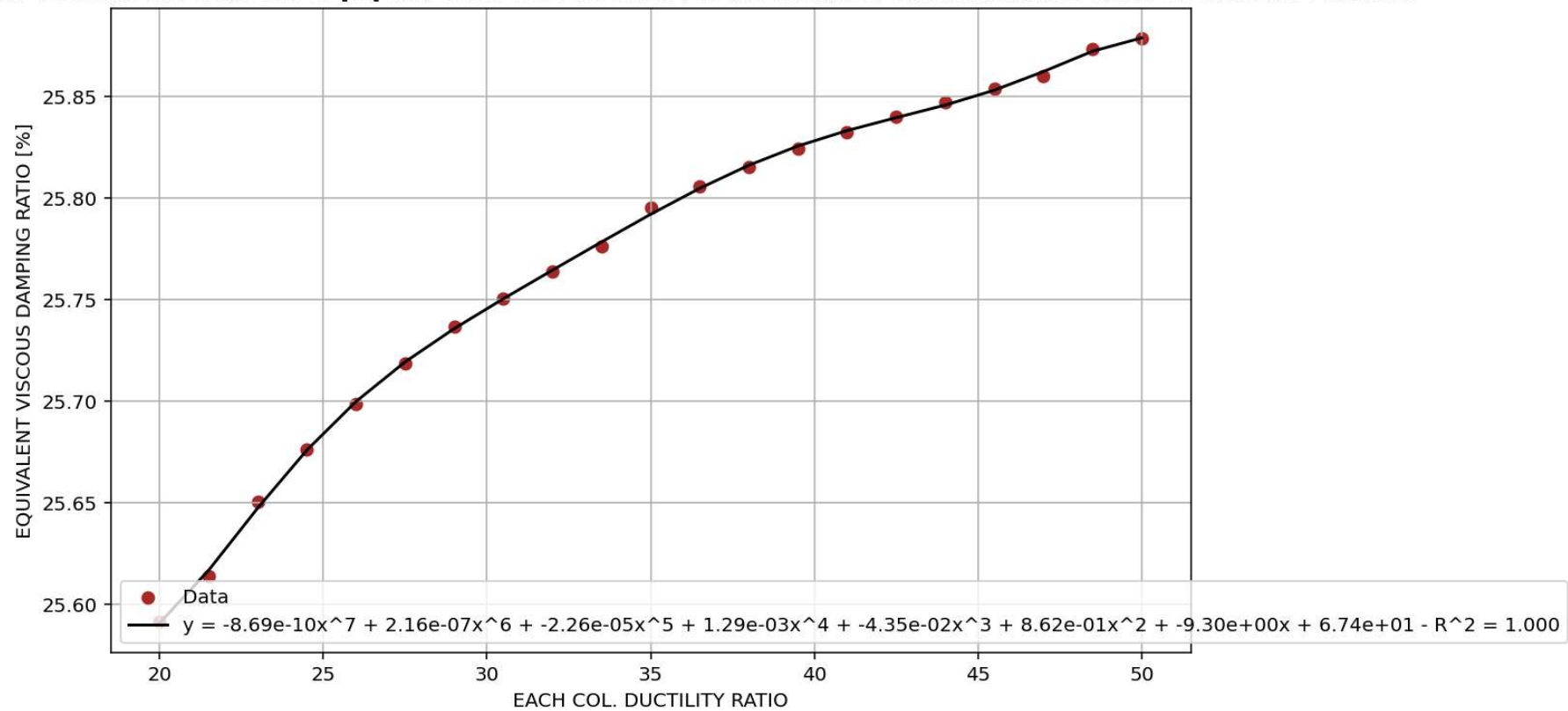
EQUIVALENT VISCOUS DAMPING RATIO [%] and EACH COL. DUCTILITY RATIO DURING PERIOD ANALYSIS WITH 20 GROUND MOTIONS
