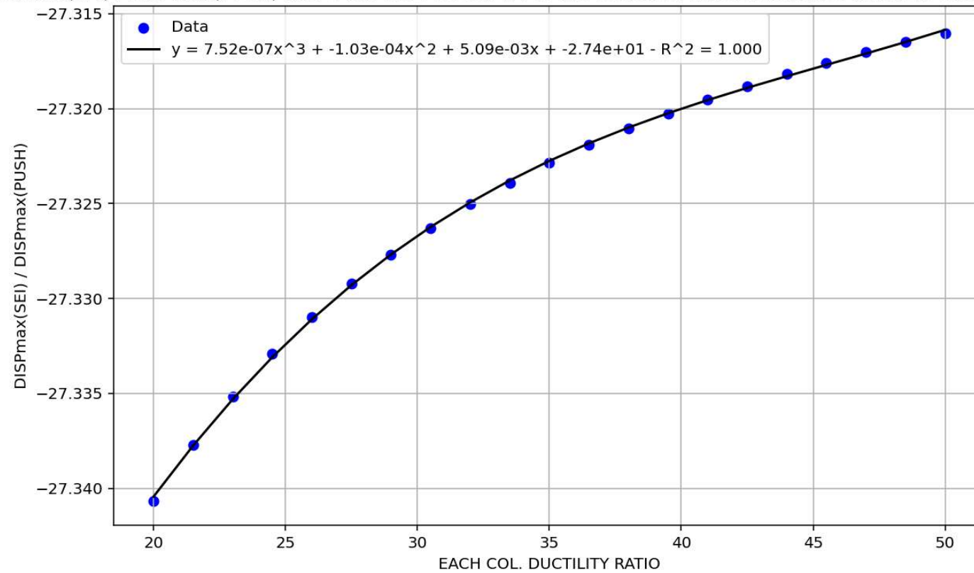
DISPmax(SEI) / DISPmax(PUSH) and EACH COL. DUCTILITY RATIO DURING PERIOD ANALYSIS WITH 20 GROUND MOTIONS
