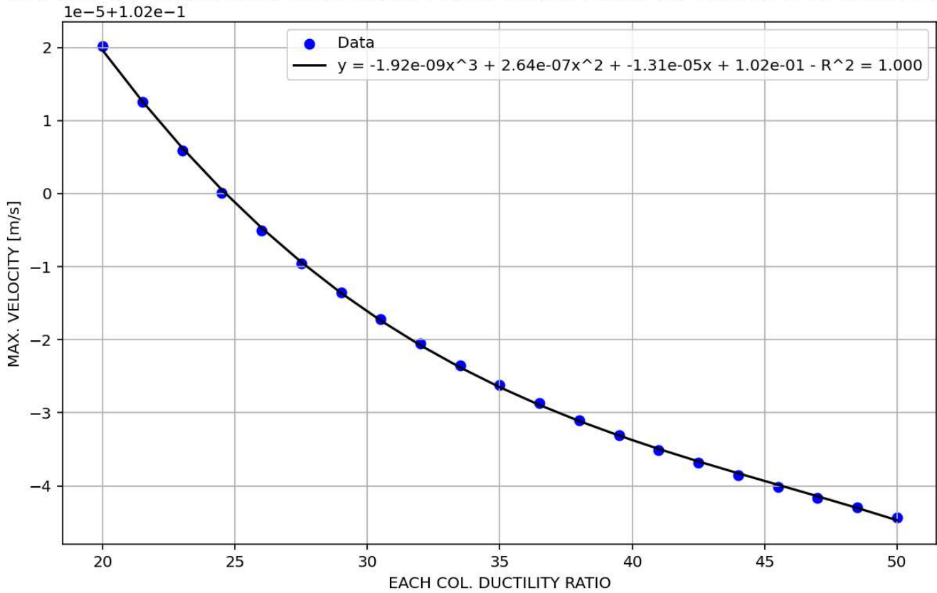
MAX. VELOCITY [m/s] and EACH COL. DUCTILITY RATIO DURING PERIOD ANALYSIS WITH 20 GROUND MOTIONS
