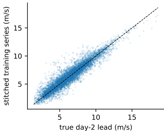
100 m wind speed, r = 0.939
