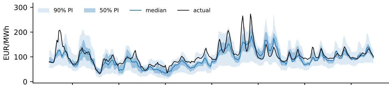
SE3, LightGBM+recal
