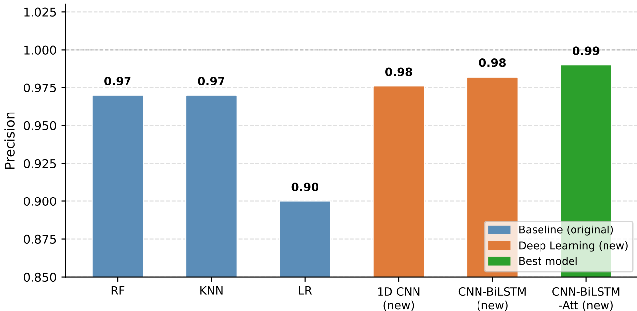
Figure 10 - Models Precisions on MIT-BIH Test (LOPO-CV)
