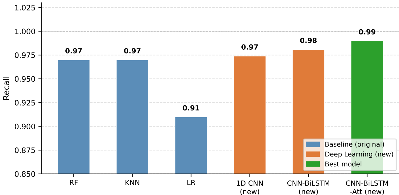
Figure 11 - Models Recalls on MIT-BIH Test (LOPO-CV)
