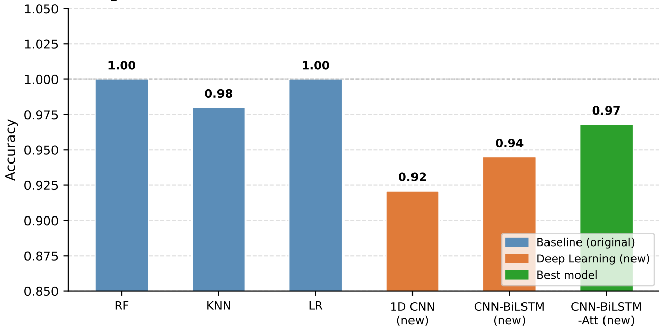
Figure 12 - Models Accuracies on PTBDB Normal (cross-dataset)
