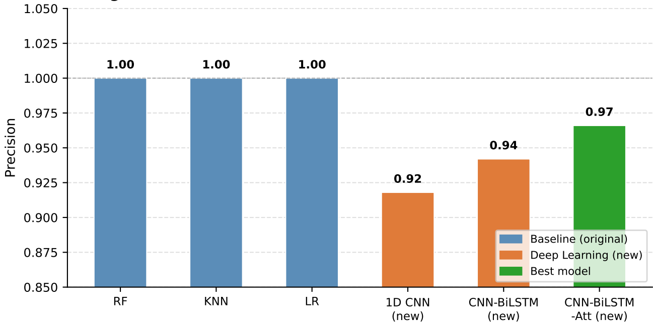
Figure 13 - Models Precisions on PTBDB Normal (cross-dataset)
