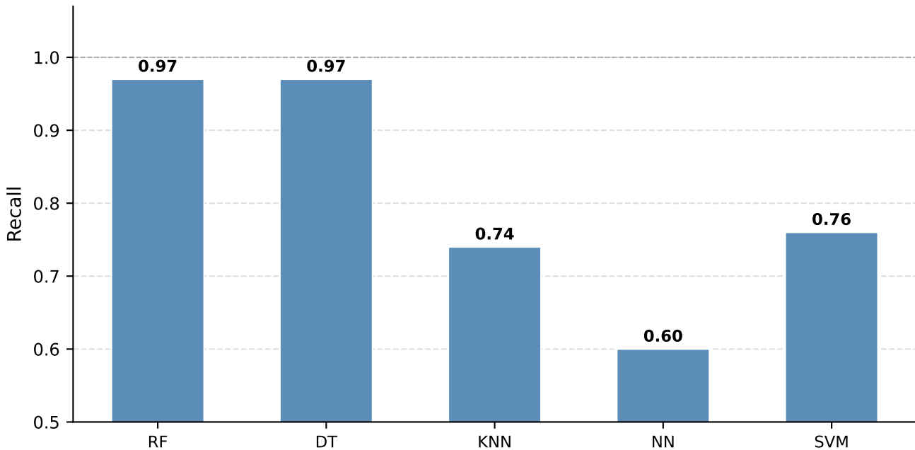
Figure 5 - Models Recalls on Heart Database
