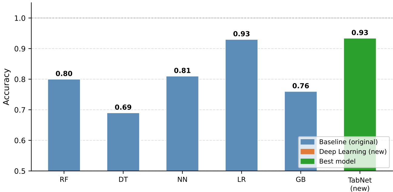
Figure 6 - Models Accuracies on HDP Database
