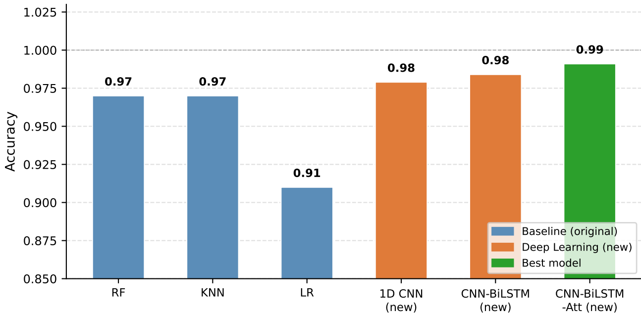
Figure 9 - Models Accuracies on MIT-BIH Test (LOPO-CV)
