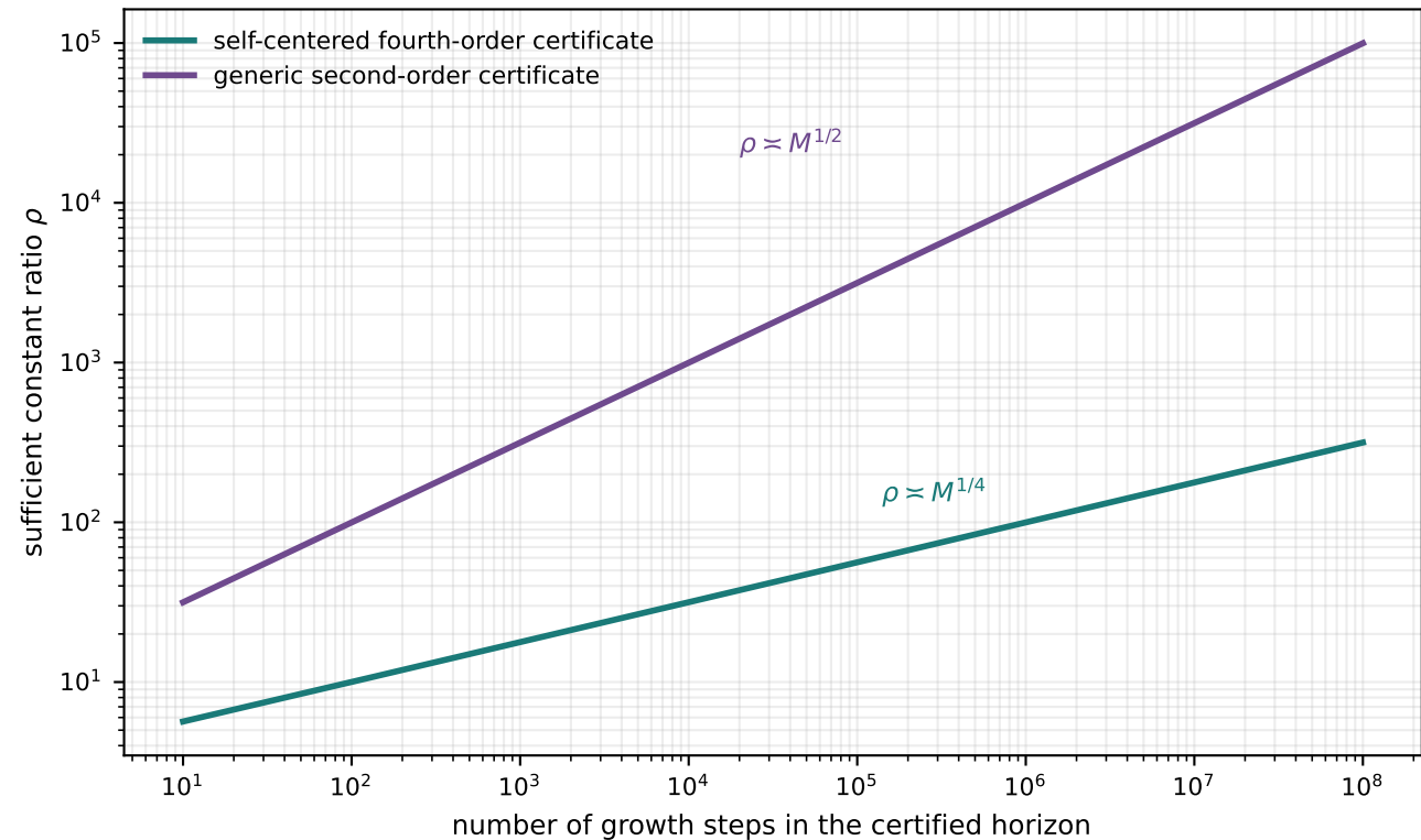
Worst-case boundary growth for a 1% path-law budget
