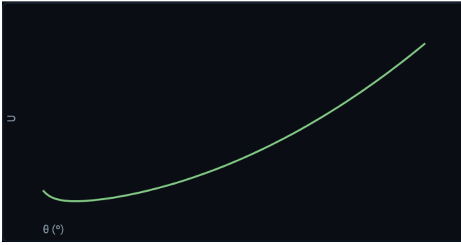
FIG. 3. U_{\text{res}}(\theta) well with \theta_c annotation; bounded nutation between turning points.
