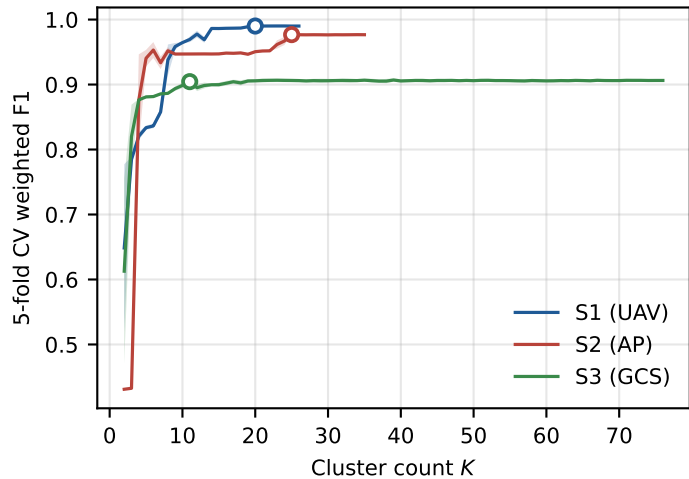
B: multi-class
