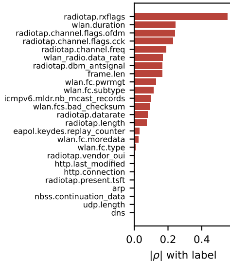
B: S2 (AP), 25 features
