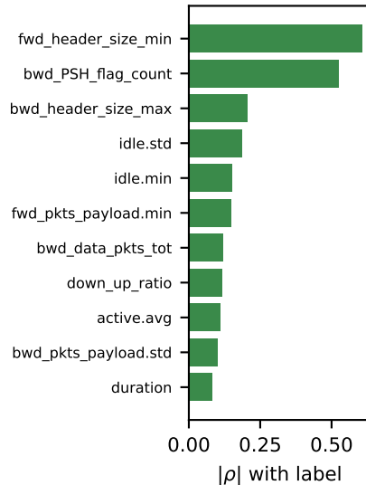
C: S3 (GCS), 11 features
