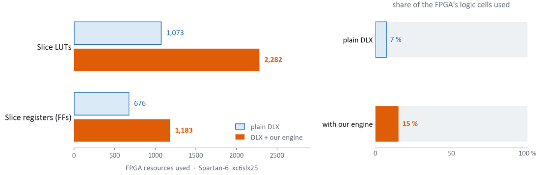
Figure 10: FPGA resources used, plain DLX against Extended DLX, and the share of the Spartan-6 xc6slx25 each occupies.
