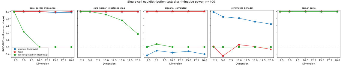
Figure 4: ROC-AUC by shape and dimension for the three refinement criteria. Random projection’s power on the two border-imbalance shapes visibly collapses toward chance as dimension grows, exactly as Theorem 2’s discussion predicts ( R(v) = \Theta(\sqrt{d}) weakens the bound); Weyl’s power does not.
