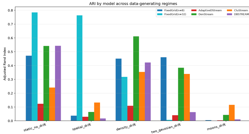
Figure 6: Adjusted Rand Index by model across the five regimes in Table 5.
