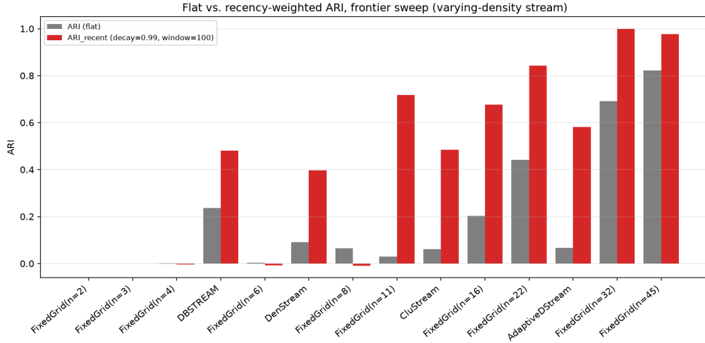
Figure 9: Flat vs. recency-weighted ARI, frontier sweep.
