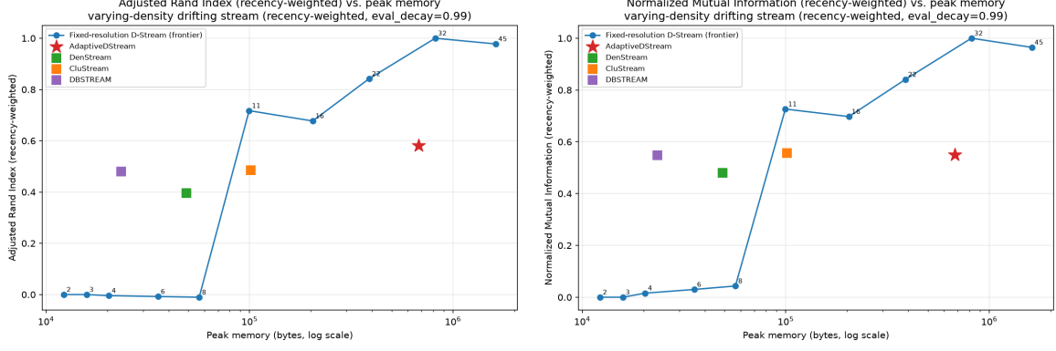
Figure 10: Recency-weighted ARI and NMI vs. peak memory, frontier sweep ( \lambda_{\text{eval}} = 0.99 ).
