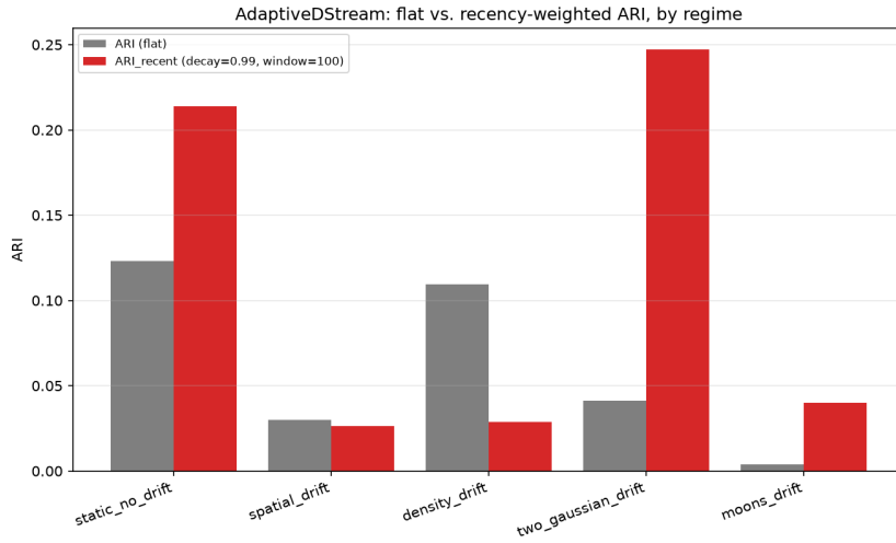
Figure 11: AdaptiveDStream: flat vs. recency-weighted ARI, by regime.
