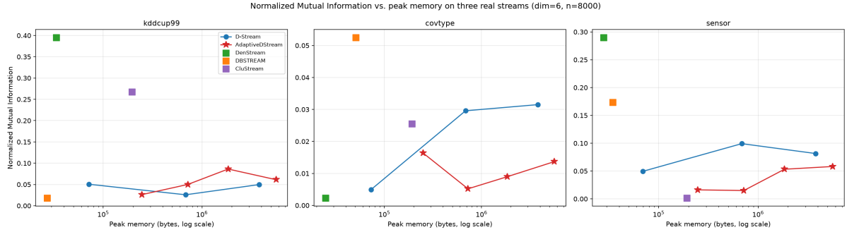
Figure 8: Normalized Mutual Information vs. peak memory (log scale), three real datasets.
