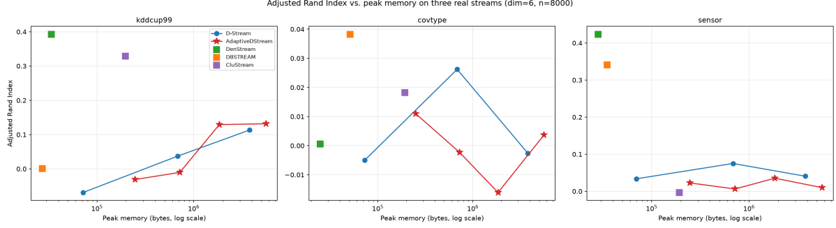
Figure 7: Adjusted Rand Index vs. peak memory (log scale), three real datasets. Circles: FixedGridDStream frontier. Stars: AdaptiveDStream frontier. Squares: river baselines.
