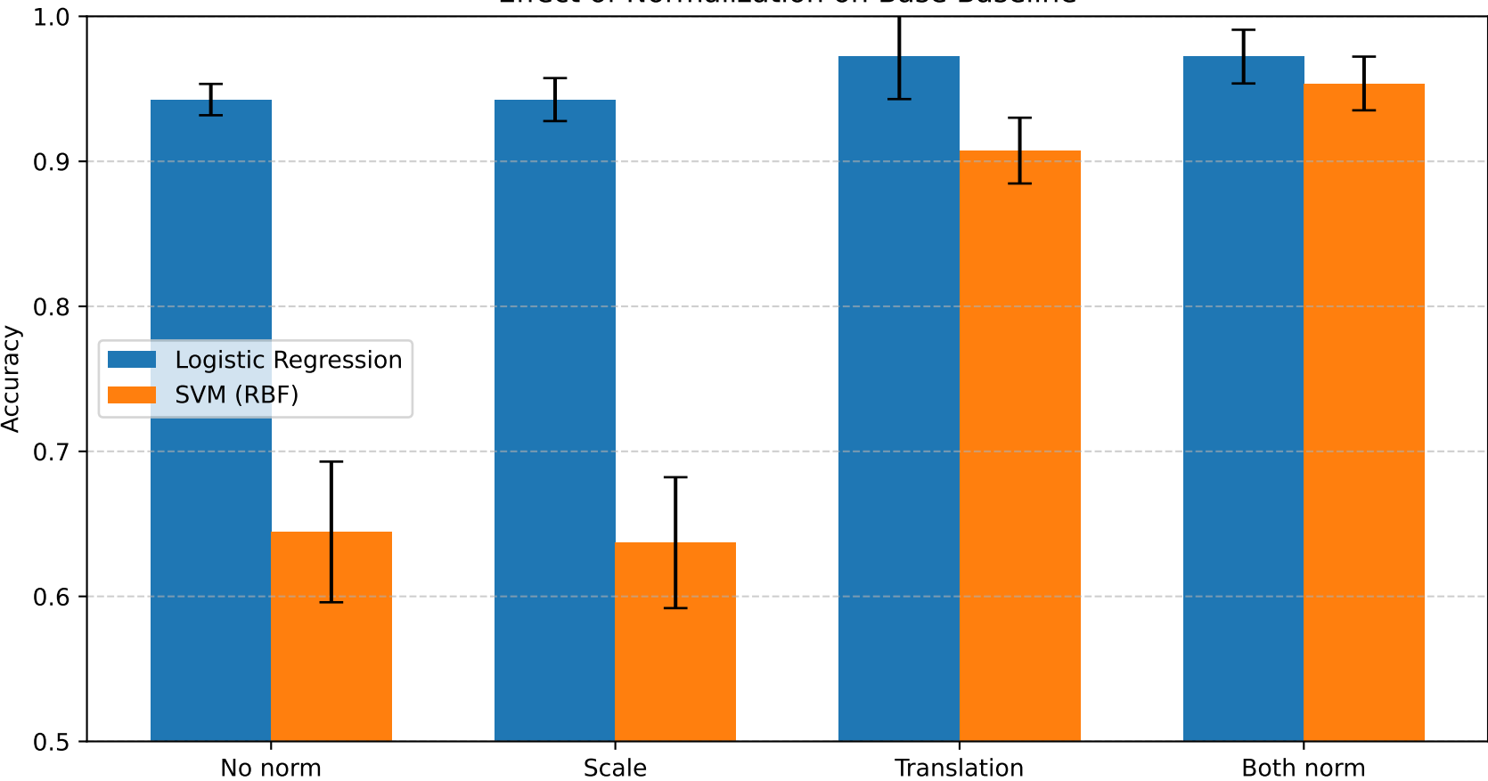
Effect of Normalization on Base Baseline
