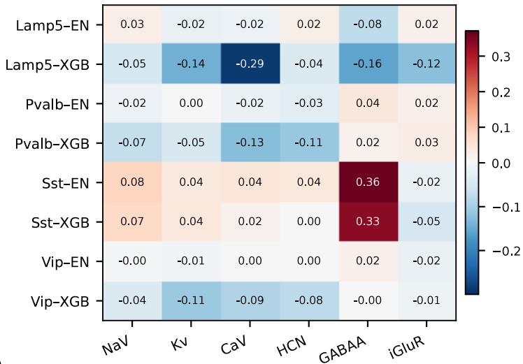
(b) Within-subclass OOF R^2
