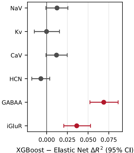
(a) Paired donor bootstrap
