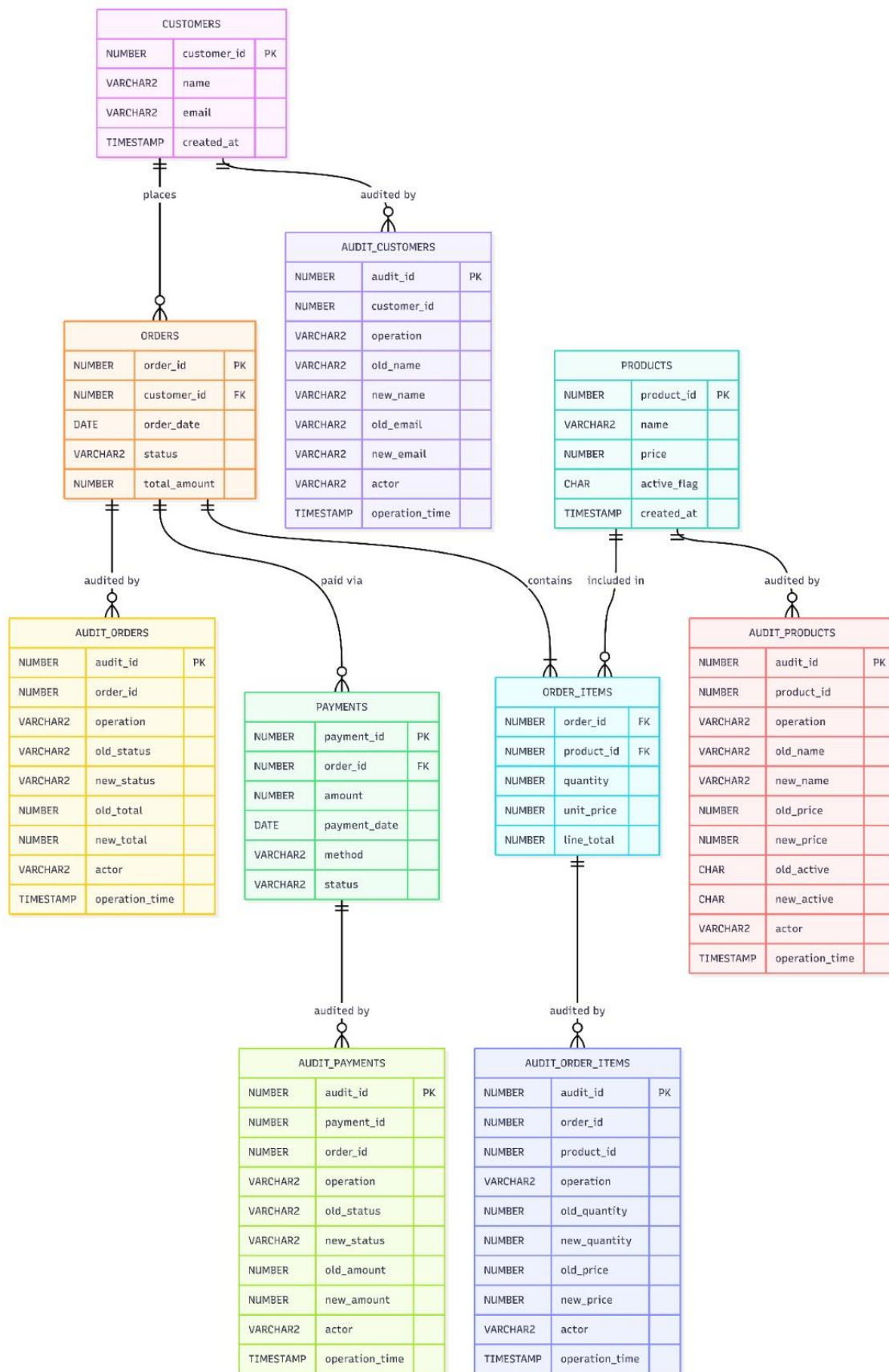
Figure 2: Complete Schema with Audit Tables
