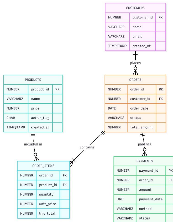
Figure 1: Entity-Relationship Diagram of the E-Commerce Schema
