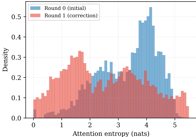
Attention Entropy Distribution
