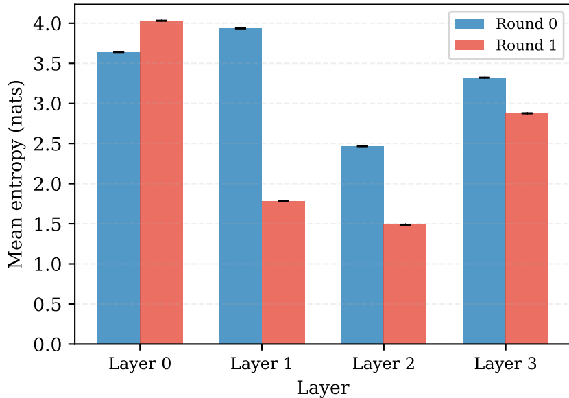
Entropy by Layer
