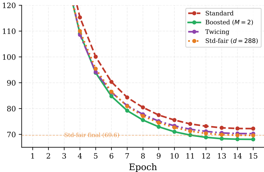
Validation Perplexity
