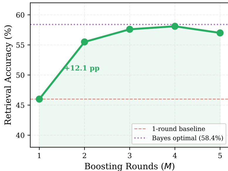
Ablation: Rounds (pattern retrieval)
