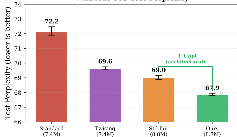
WikiText-103 Test Perplexity
