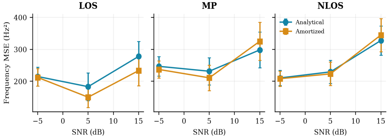
Figure 2. Mean frequency MSE by SNR, channel, and architecture; bars are 95% seed-block t intervals.
