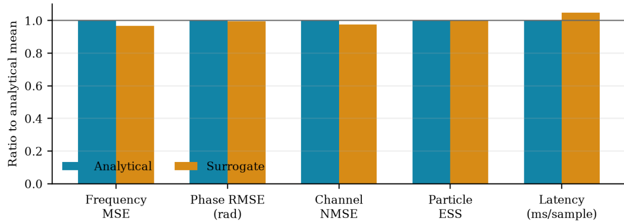
Figure 1. Endpoint means expressed relative to the analytical architecture.
