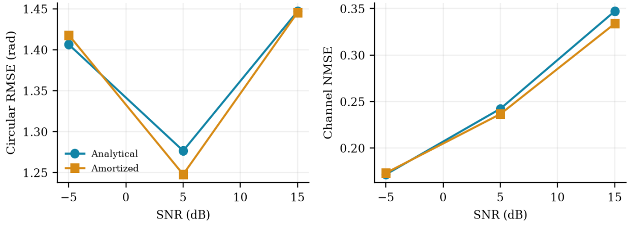
Figure 3. Circular phase RMSE and complex channel NMSE by SNR and architecture.
