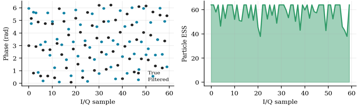
Figure 7. Analytical torus phase and particle ESS for the same trace.
