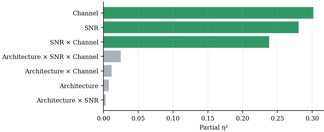
Figure 5. Partial eta squared for omnibus effects on log frequency MSE; green effects survive Holm adjustment.
