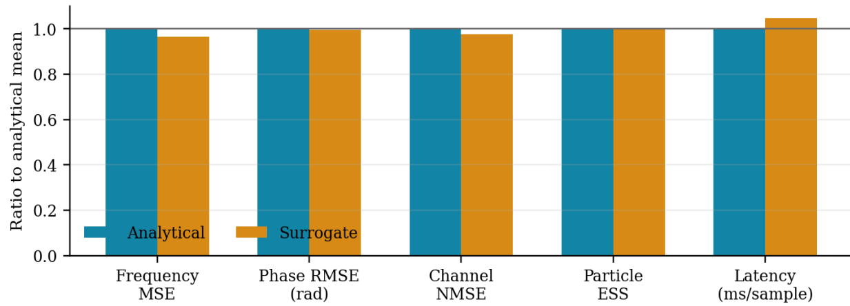
Figure 1. Endpoint means expressed relative to the analytical architecture.
