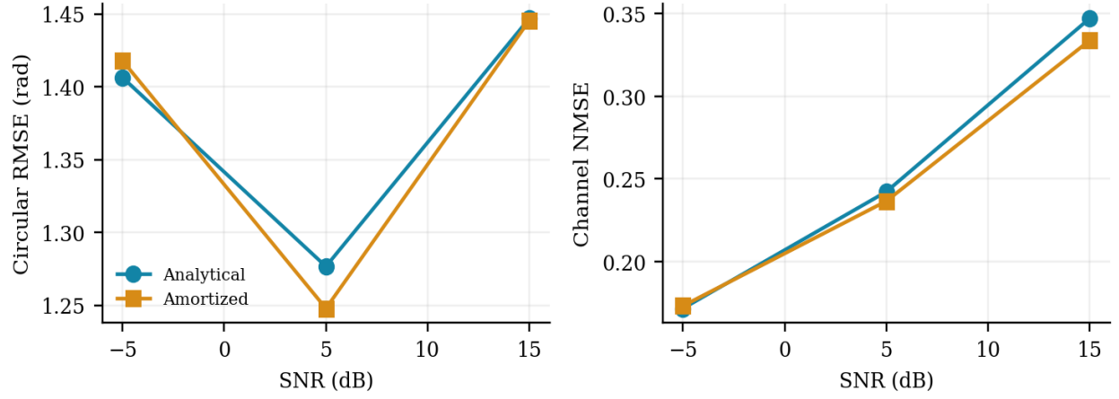
Figure 3. Circular phase RMSE and complex channel NMSE by SNR and architecture.
