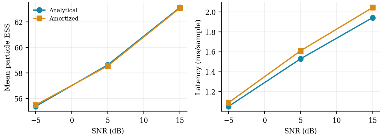
Figure 4. Mean particle ESS and software latency by SNR and architecture.
