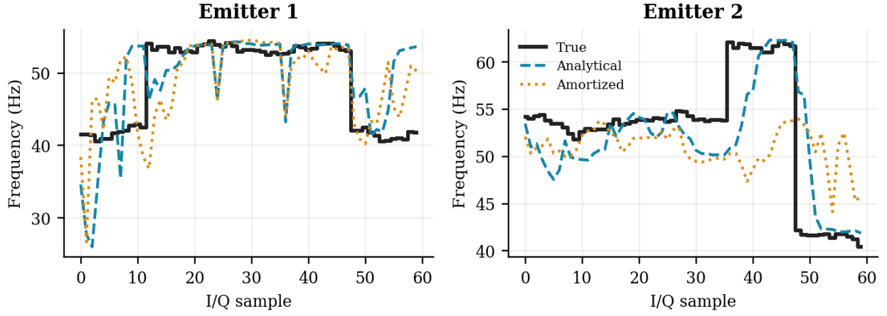
Figure 6. Predeclared seed-0, +5 dB NLOS frequency trace.
