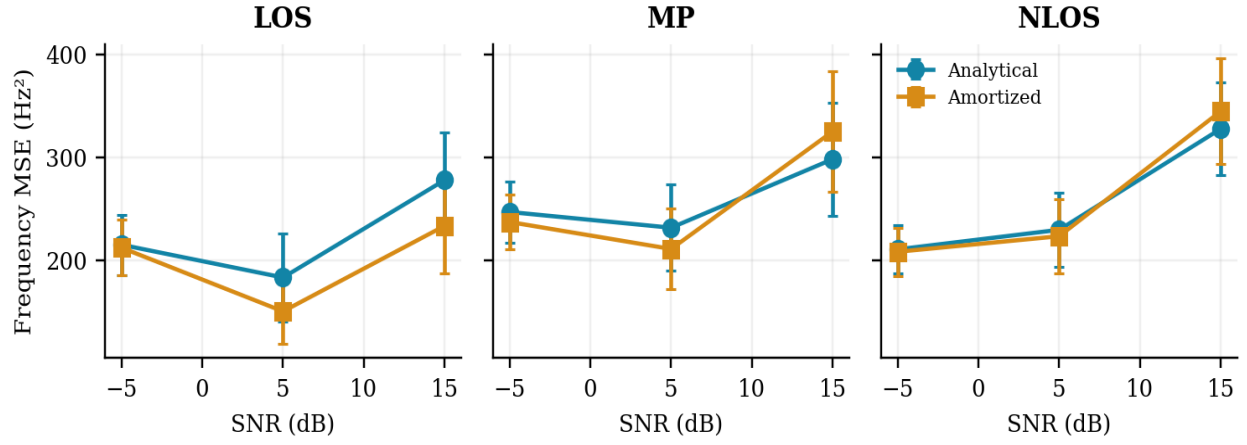
Figure 2. Mean frequency MSE by SNR, channel, and architecture; bars are 95% normal intervals.
