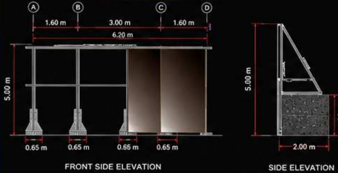
PLANS - 5 METER
