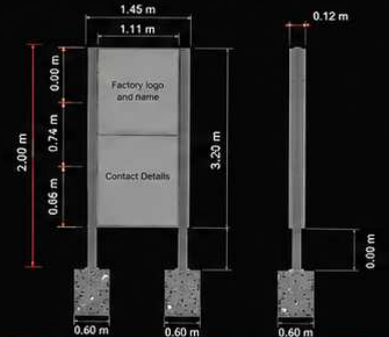
CITY LIGHT BOX PLAN
