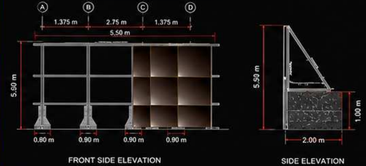
PLANS - 5.5 METER
