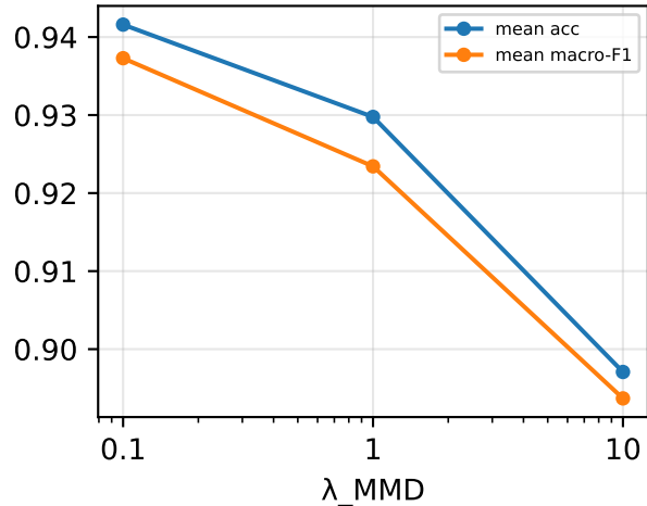
Source validation
