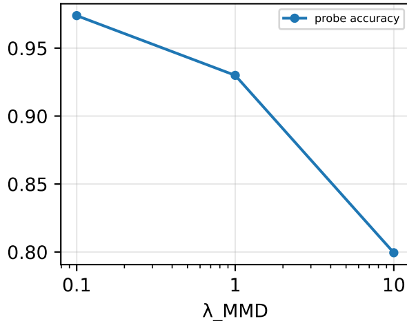
Domain separability
