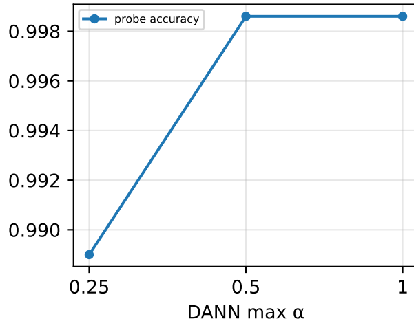
Domain separability
