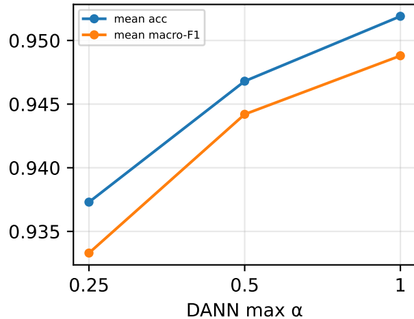
Source validation
