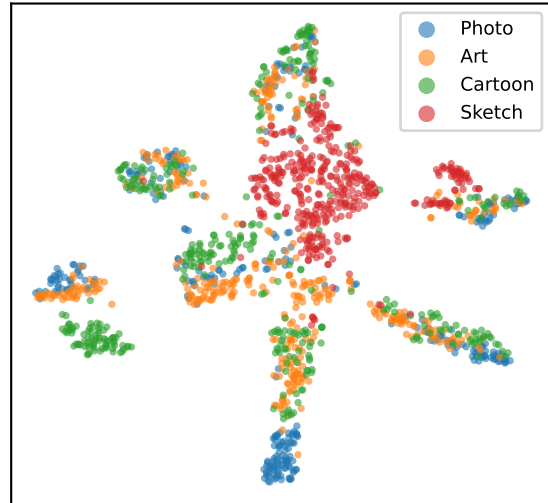
source_only
