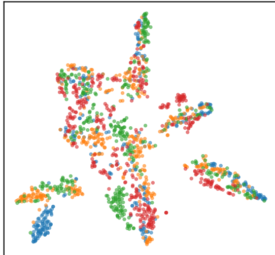
cdan
