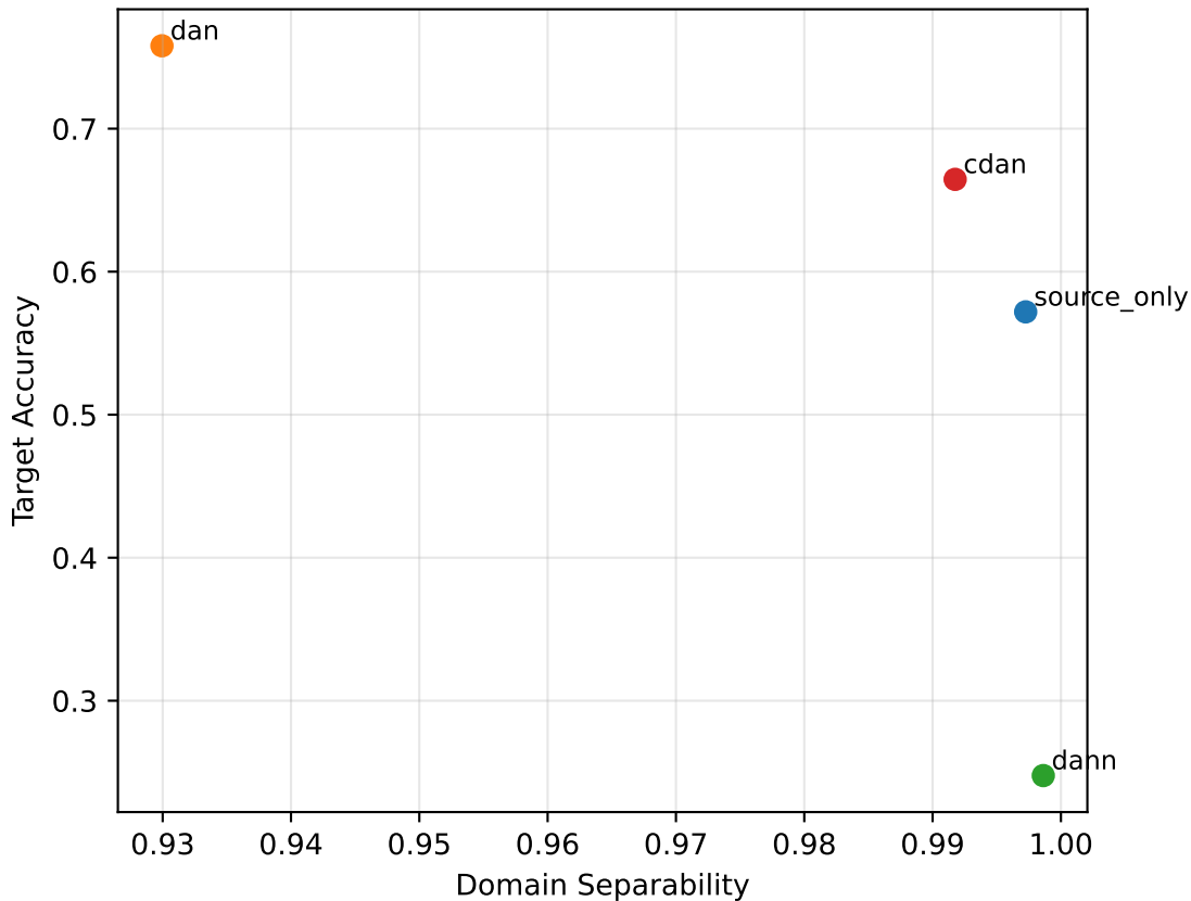
Task 2: domain separability vs. Sketch accuracy
