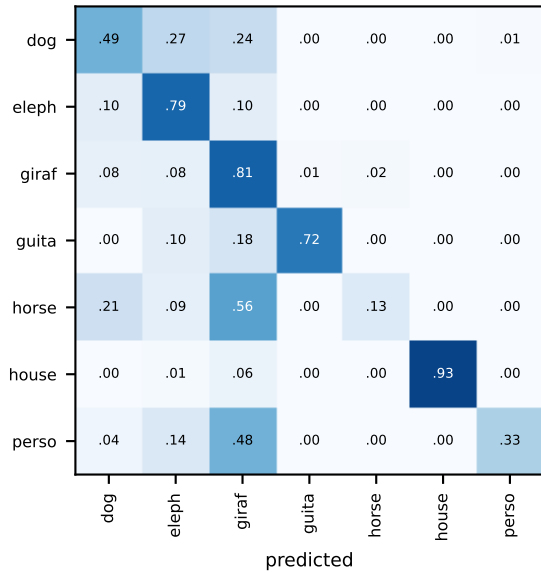
source_only (acc 0.572)
