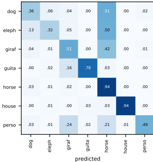
dan_dg (acc 0.585)
