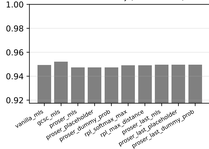
Closed-set accuracy (CIFAR-10 test)
