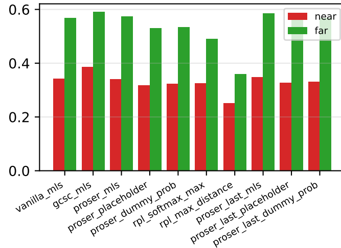
Rejection @ \tau (95% val acceptance)
