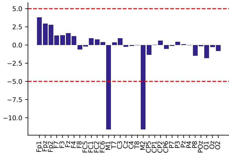
Variance z-score
