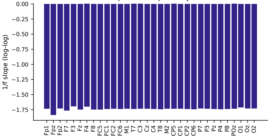
Per-channel aperiodic slope · Subject 1 Eval-6
