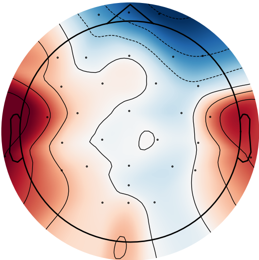
TRF topomap at -100 ms
