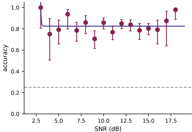
F2 · Psychometric curve (all subjects pooled)
