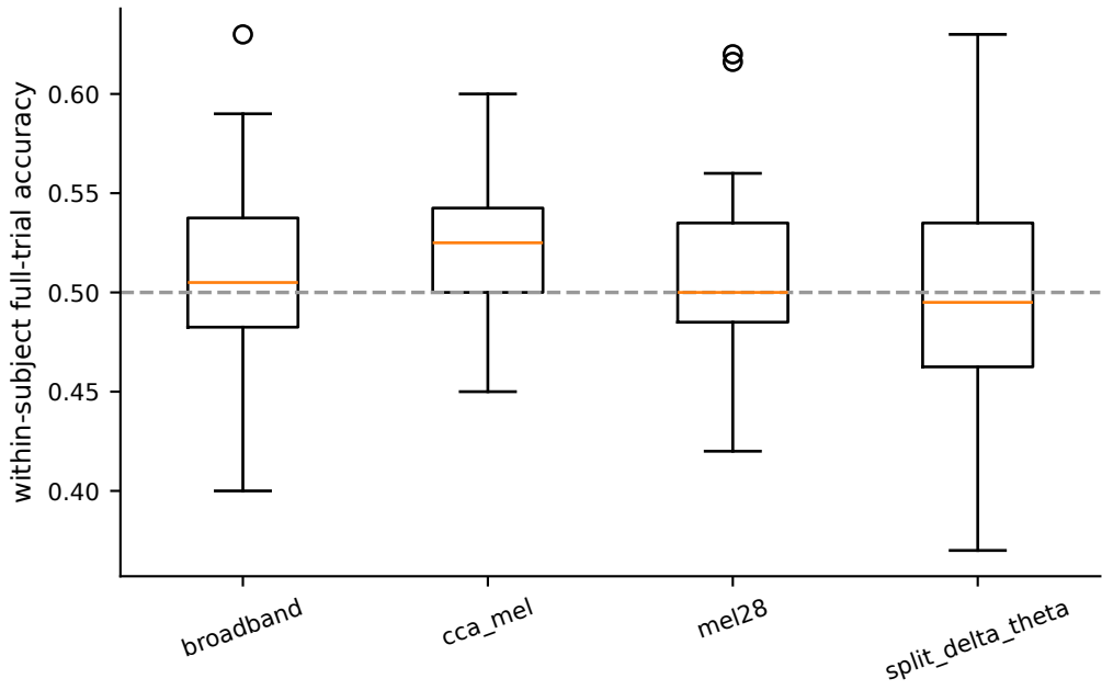
iter-3 · backbone comparison (per-subject distributions)
