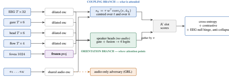
Figure 1: MERIT . The coupling branch compares the EEG with each candidate using a correlation over time with the mean removed. A brain encoder that outputs the same vector at every step therefore gives every candidate a score of zero, which is chance. The orientation branch gets no audio , so it cannot use audio cues. The model encodes once and scores separately, so a trained model can be re-scored under any shuffle of any stream without encoding again.
