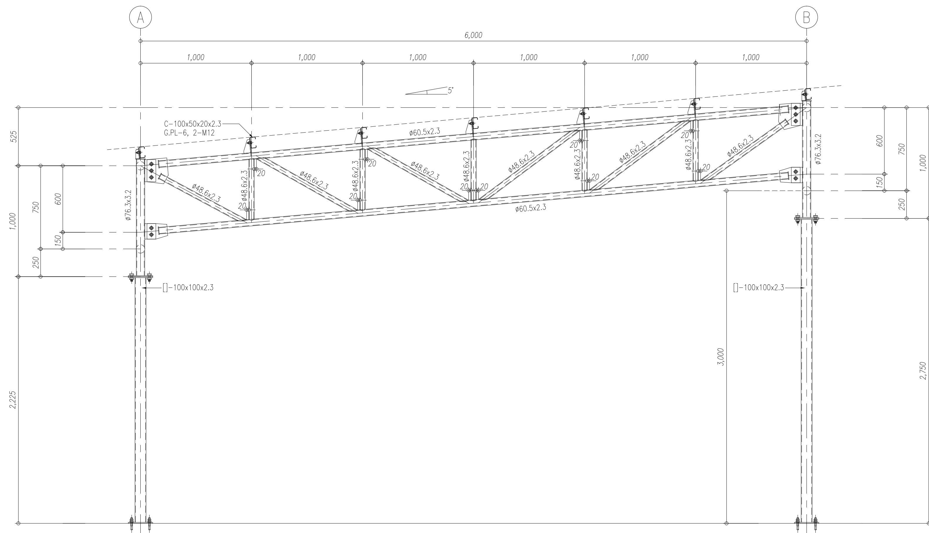
FRAMING ELEVATION LINE 1 SCALE 1/20
