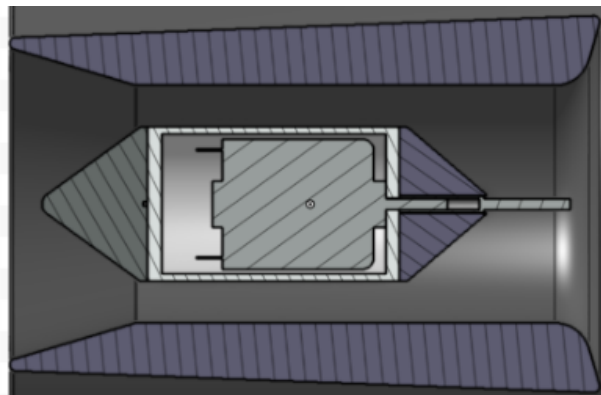
Figure 2. Cross-sectional geometry of the optimized Venturi tube.
