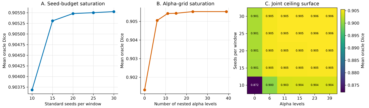
Figure 4: Practical saturation of candidate capacity. Seed and fuzzy \alpha -cut budgets were enlarged in nested fashion. Every value is a retrospective pool-oracle mean Dice and is unavailable to the label-free selector.
