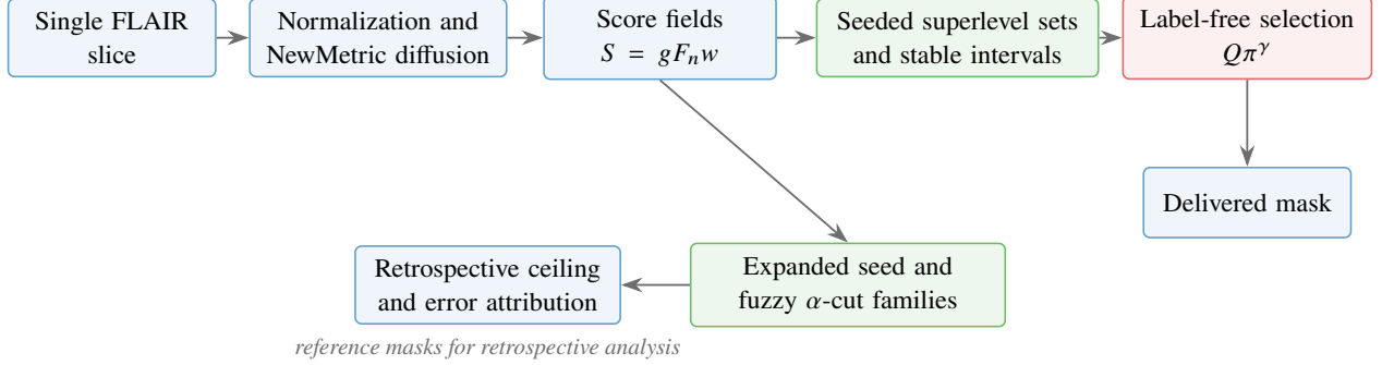
Figure 1: Study method and analytical separation. The upper sequence produces the label-free segmentation. Expanded seed and fuzzy \alpha -cut families are evaluated only to measure candidate capacity and attribute errors; they do not replace the primary delivered mask. Reference masks are also used earlier for TCGA parameter development and prespecified slice selection, as detailed in Section 3.1.
