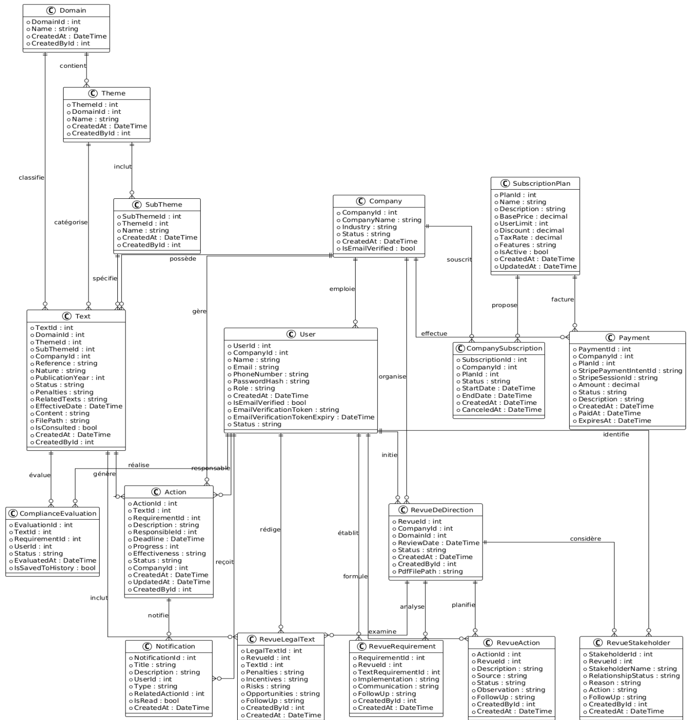
FIGURE 2.2 – Diagramme des classes global
