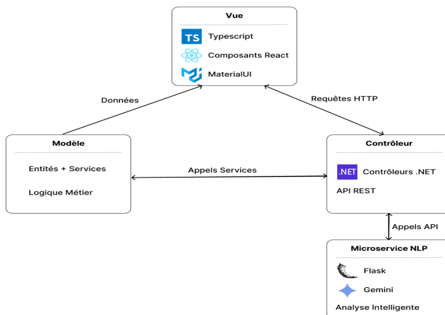
FIGURE 3.13 – Architecture logique de l'application
