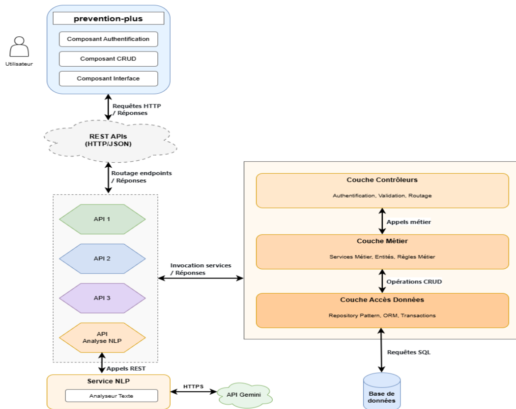
FIGURE 3.13 – Architecture logique de l'application
